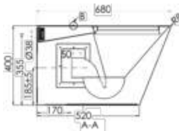
Cross Section
