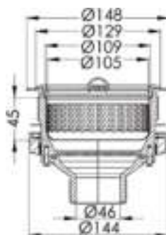
Cross Section
