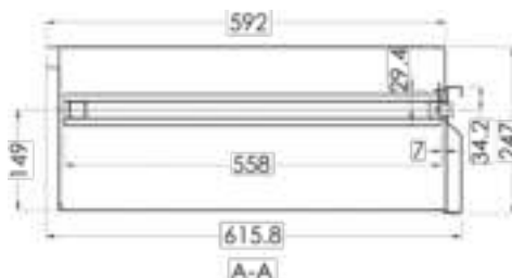
Cross Section
