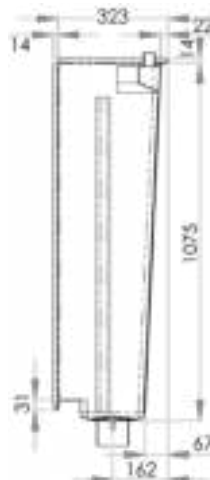
Cross Section
