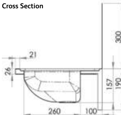
Cross Section
