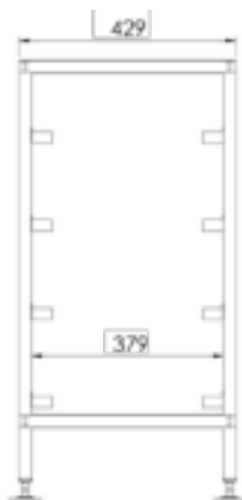
BRK-C
