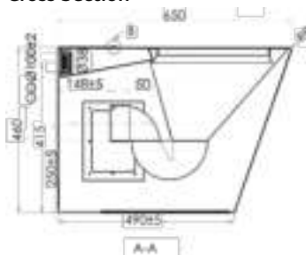
Cross Section
