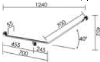
CF-454-SS
