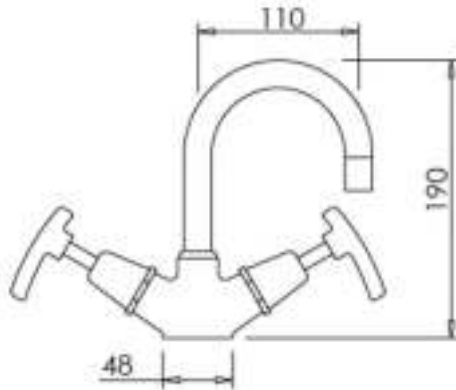
T-3MTWIN-B
