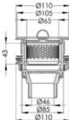
SCRAP-S-90-P-316
