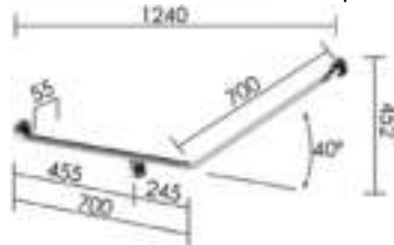
CF-454-SS
