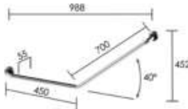
CF-877-LH-SS / CF-877-RH-SS (left hand shown)
