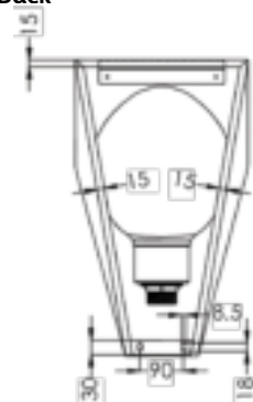
Bracket
