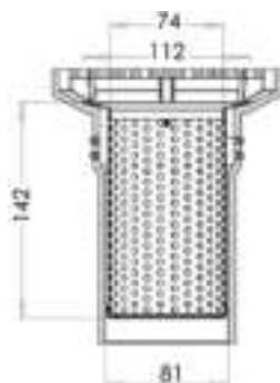
Cross Section
