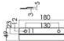
Floor Clip
