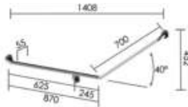
CF-966-LH-SS / CF-966-RH-SS (left hand shown)
